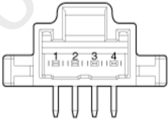
Connector A
